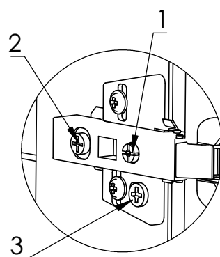
DETAIL L
