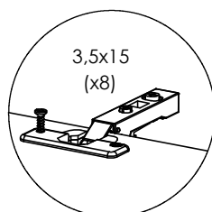
DETAIL E
