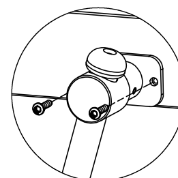
DETAIL 4
