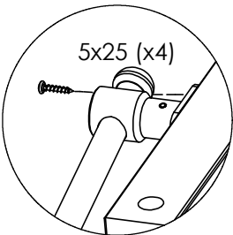
DETAIL G
