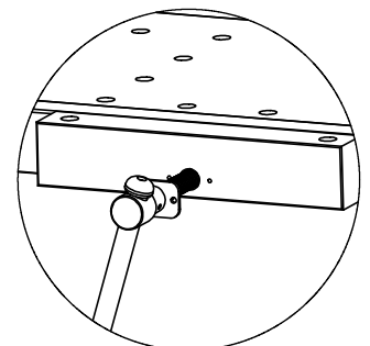
DETAIL 3
