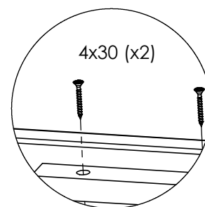
DETAIL I
