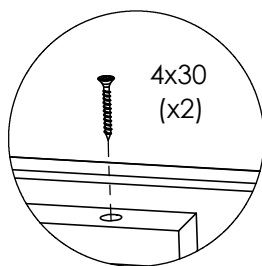
DETAIL H
