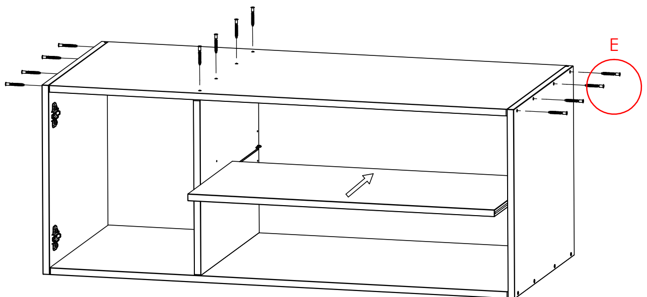
DETAIL E
